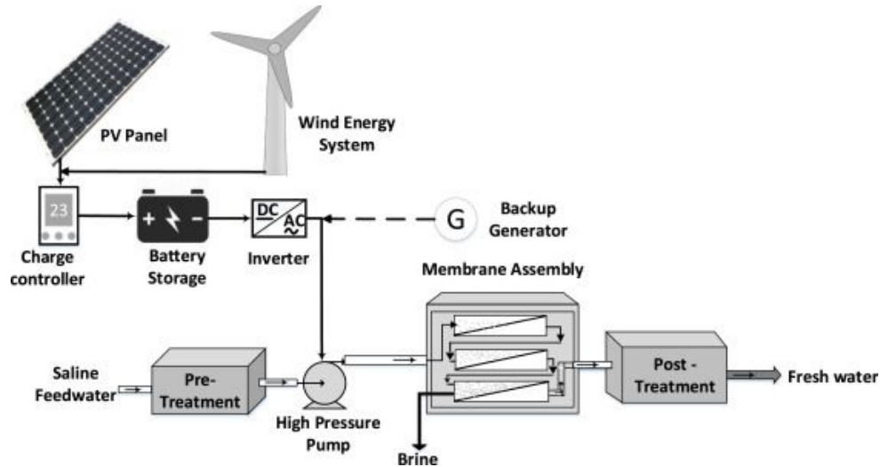
Figure 6. Water desalination using reverse osmosis powered by a hybrid renewable energy system. Taken from the Renewable and sustainable energy review journal .
